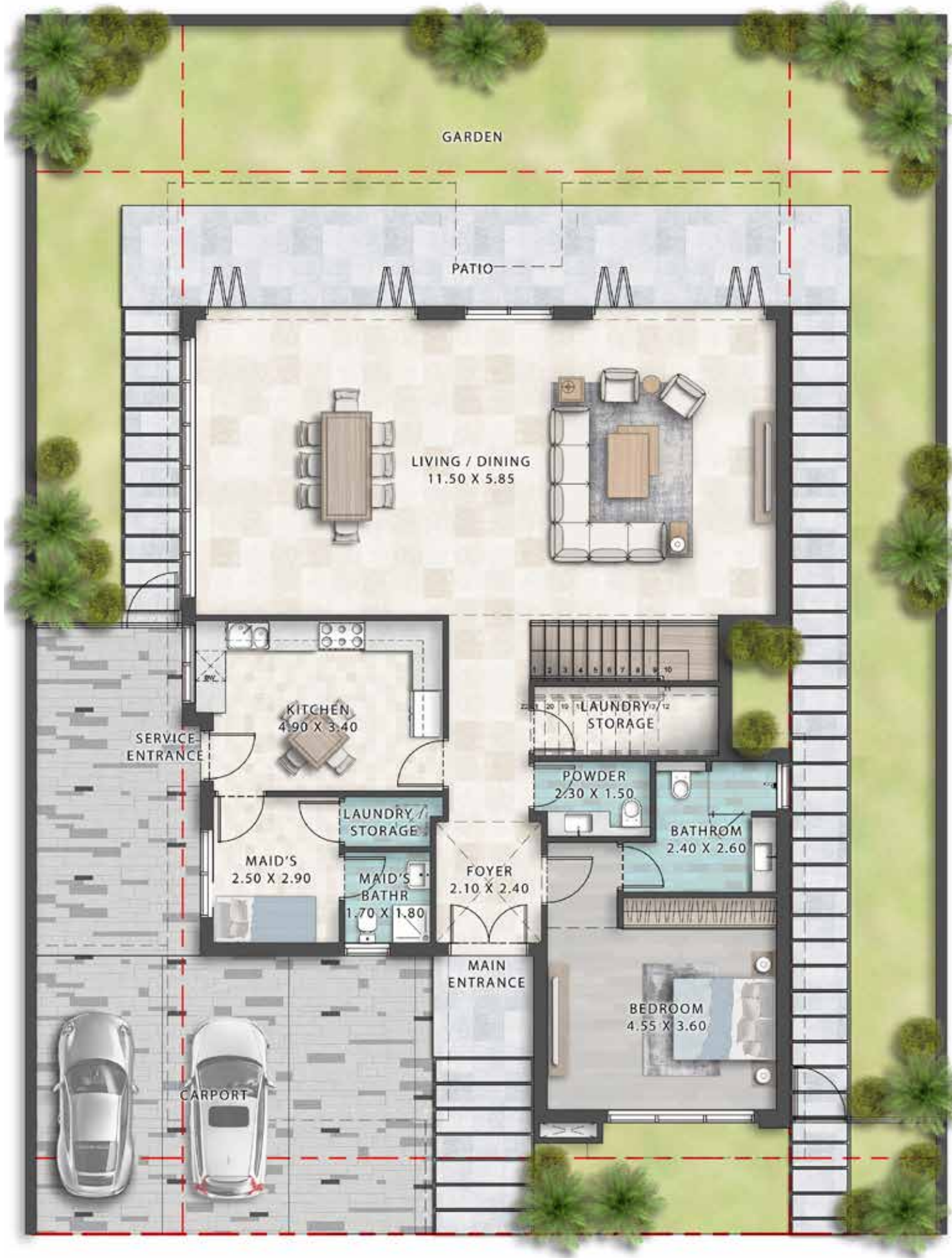
GROUND FLOOR
